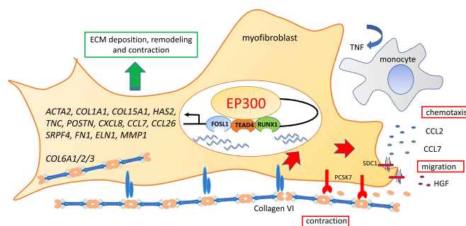
Fig. 5. Schematic illustrating the epigenetic control by EP300 of the profibrotic phenotype of myofibroblasts in Dupuytren's disease. Persistent activation of EP300 acetylates histones and transcription factors to promote extracellular matrix production and myofibroblast contractility. Collagen VI, a key target of EP300, plays a dominant role in regulating contraction. Proteolytic cleavage by PCSK7 generates small bioactive collagen VI fragments which control recruitment of immune cells by chemokine production, thereby perpetuating the cycle of chronic inflammation and fibrosis by the secretion of cytokines such as TNF.
