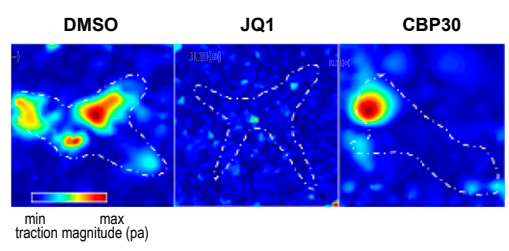
Fig. 1. CREBBP/EP300 regulates profibrotic gene expression and contractile phenotype in myfibroblasts. (A) Pi analysis identifies CREBBP and EP300 as highly ranked central network genes in DD. Target pathway crosstalk for DD is shown, maximizing numbers of highly prioritized interconnecting genes. (B) Epigenetic probe library screening of ACTA2 , COL1A1 , COL3A1 , and TGFB1 gene expression in DD patient-derived myfibroblasts. Cells were incubated with probes for 3 d. Gene expression was analyzed by Taqman qPCR using the \Delta\Delta Ct method, normalized to GAPDH . Data are means \pm SEM of five independent experiments from five individual donors, represented as a heatmap where values are normalized to DMSO control value; 100% represented in white, red represents inhibition and blue represents augmentation of gene expression relative to control. (C and D) Data from heatmap where the most potent inhibitory probes are depicted graphically; mean \pm SEM from five donors. P value was determined by one-sample t test to normalized control (DMSO) sample of value of 1. * P \leq 0.05, ** P < 0.01, *** P < 0.001, **** P < 0.0001. ChIP-qPCR analysis of JQ1 (0.5 \mu M) and SGC-CBP30 (2.5 \mu M) inhibition of the H3K27ac mark at promoter proximal regions of ACTA2 (E) and COL1A1 (F) in patient-derived myfibroblasts. Data are representative of three independent experiments from three individual donors, mean \pm SD of technical triplicates. Myfibroblasts were plated onto 2.55-kPa hydrogels for traction force microscopy in the presence of the indicated bromodomain inhibitors for 72 h. Color scale in stiffness maps indicates shear modulus in kilopascals. (G) Representative traction vector maps, (H) peak traction, and (I) average traction are depicted (mean \pm SEM; n = 4 independent experiments with a minimum of 20 independent cells per condition; ** P < 0.01 and * P < 0.05 versus controls).
